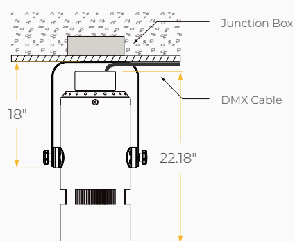
Yoke Mount
