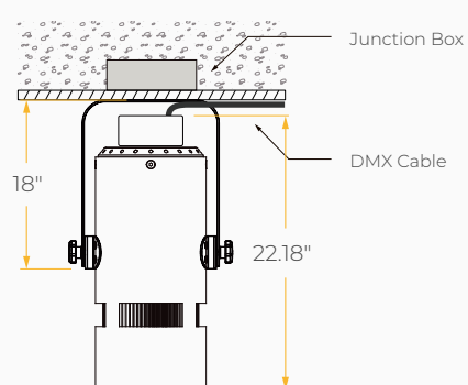
Yoke Mount
