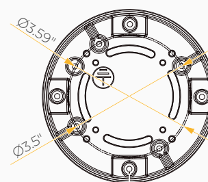
#10-32 Thread Size UNF x9
