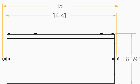
Remote Power Box
