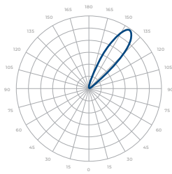
30° INDIRECT
