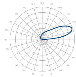
ASYMMETRIC INDIRECT
