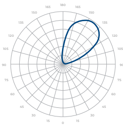
60° INDIRECT
