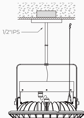
Stem Mount
