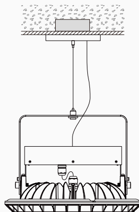
Adjustable Cable Mount
