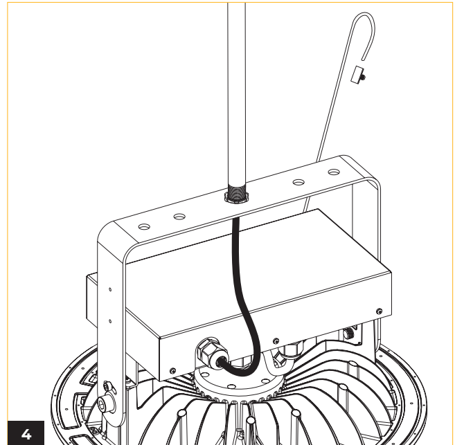
4 Clasp the hook onto the allocated bolt on the fixture mount.
