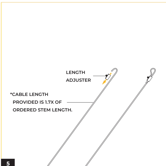
5 Loop the aircraft cable through the mounting corners and tighten the clamp by adjusting the screw. Ensure that the height is adjusted before tightening the clamp.
