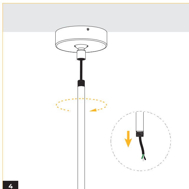
4 Thread AC wire through stem and fasten to swivel ball.
