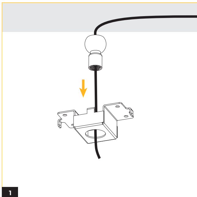
1 Thread AC wires through swivel ball and mounting plate.
