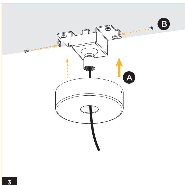
3 (A) Mount canopy onto mounting plate.
