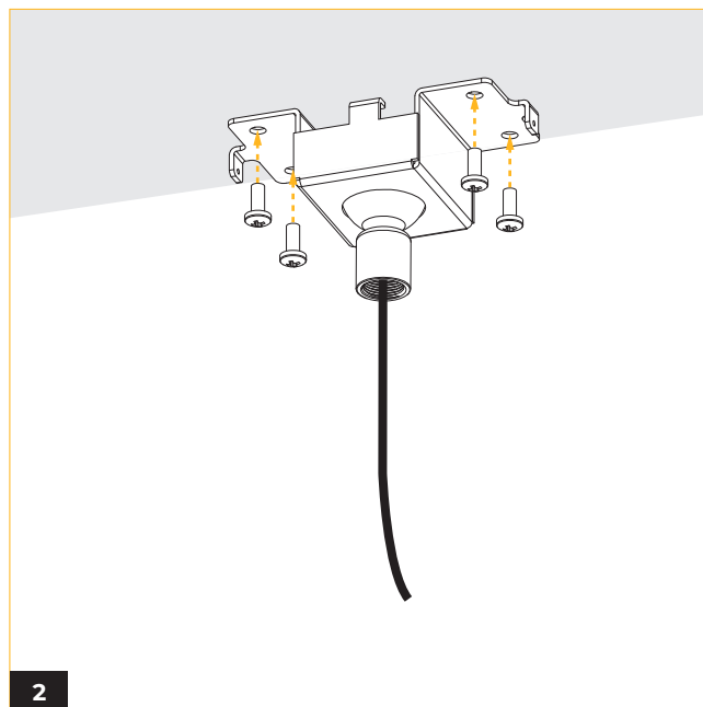
2 Mount the mounting plate and swivel ball onto flat surface using screws.
