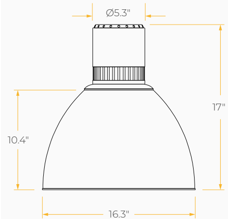
16" Shrouds
